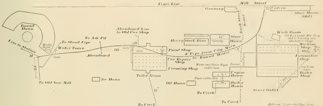
GENERAL PLAN OF ERIE SHOPS AND ROUNDHOUSE.
